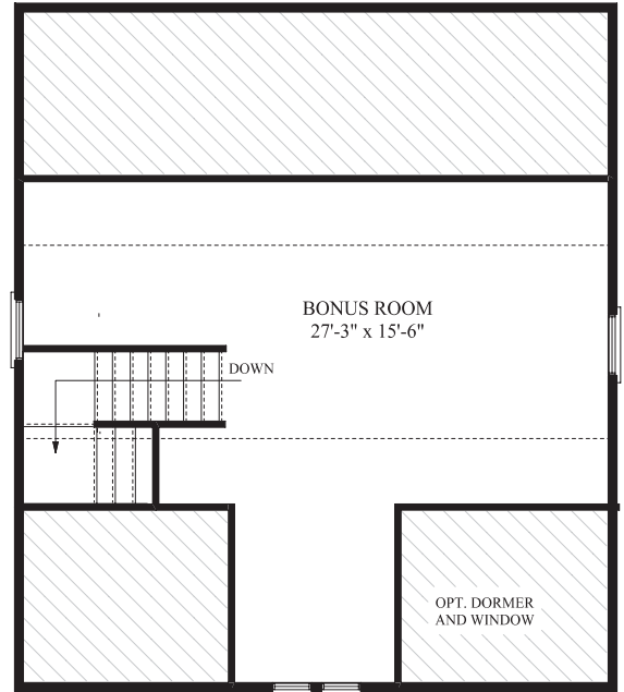
OPT. THIRD FLOOR PLAN (512 S.F.)
